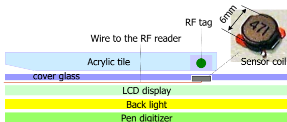
Figure 11: Cross section view of the tile tray.
